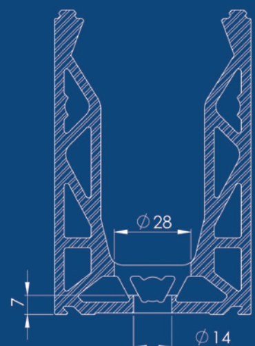
SECTION D-D Base Mount
